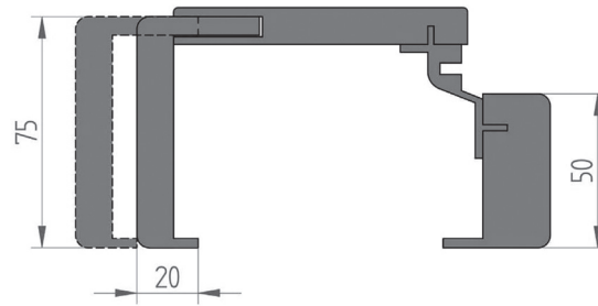
Overlay frame adjustment range (ON) and overlay tunnel frame (TN)
