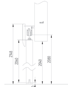
On-wall sliding system without mask
