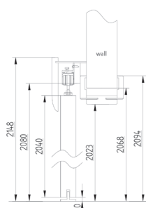
On-wall sliding masked system
