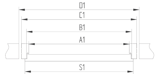
Dimensions of fixed frames (OS)
