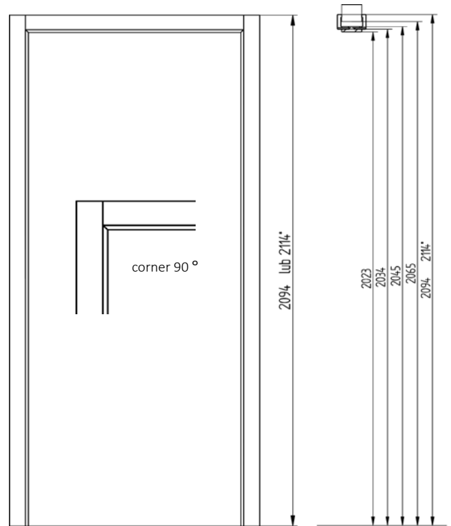
E2* - dimension for TW
