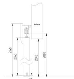
On-wall sliding system without mask
