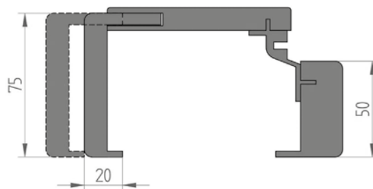
Overlay frame adjustment range (ON) and Overlay tunnel frame (TN)
