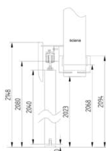
On-wall sliding system masked
