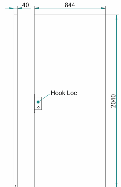
sliding leaf
