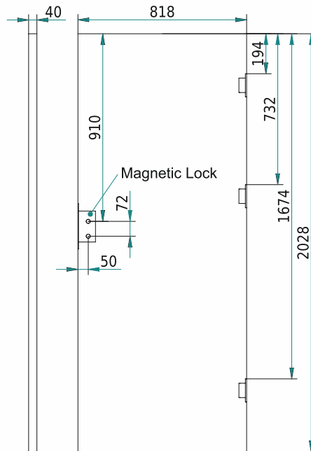
non-rebate leaf
