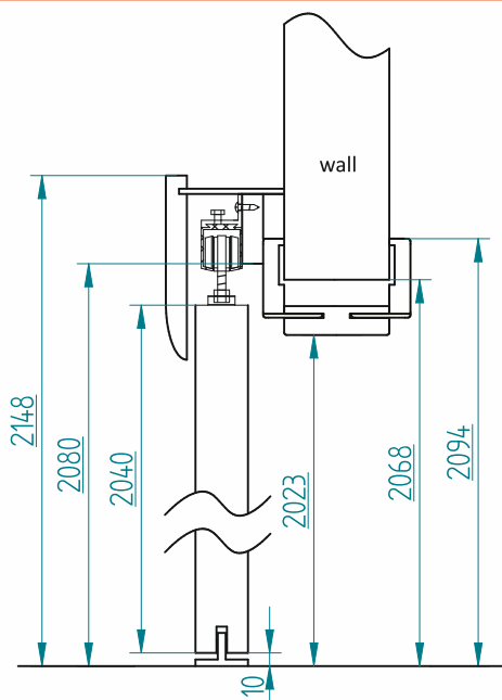
wall sliding system with encasing
