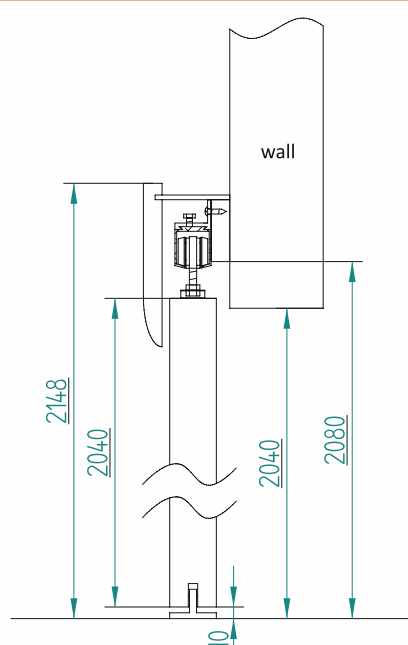
wall sliding system without encasing
