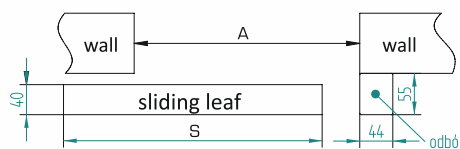
wall sliding system without encasing
