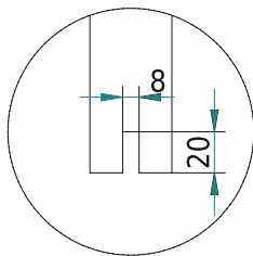
cut off of sliding leaves
